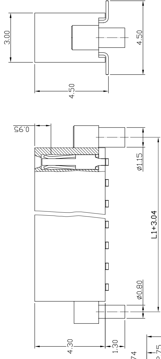
THREE SIDE CONTACT TERMINAL
